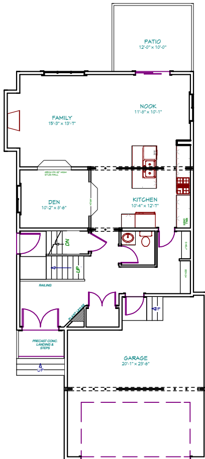
MAIN FLOOR : 955 SQ.FT.
