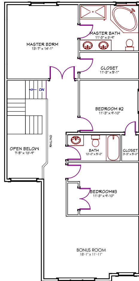
SECOND FLOOR : 1075 SQ.FT.
